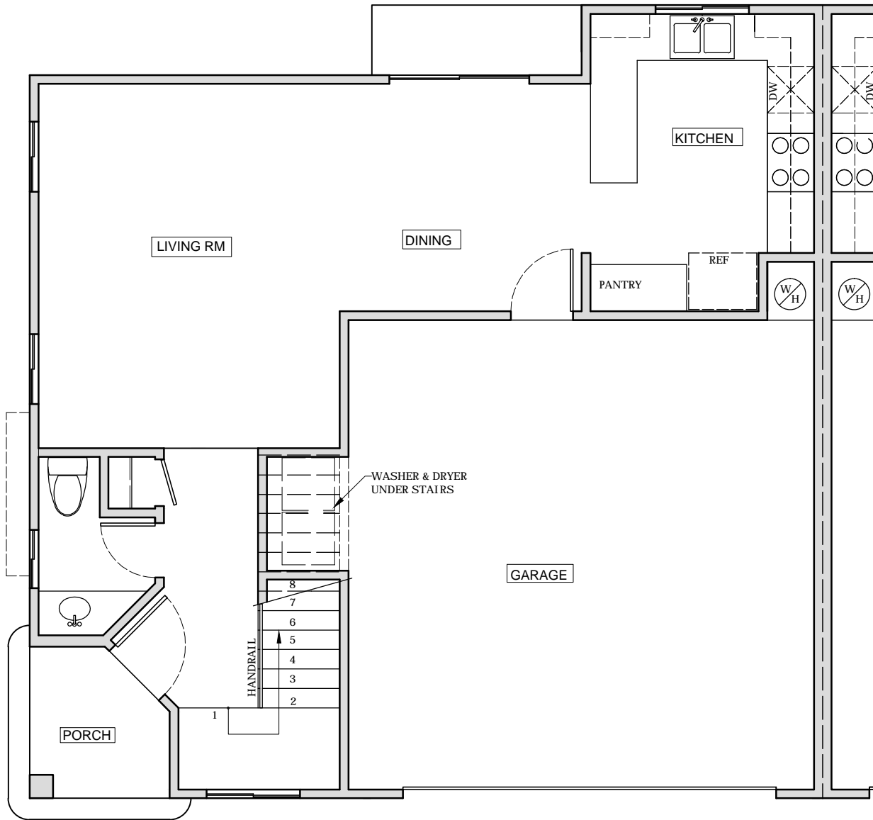
1st. LEVEL TYPICAL END UNIT
