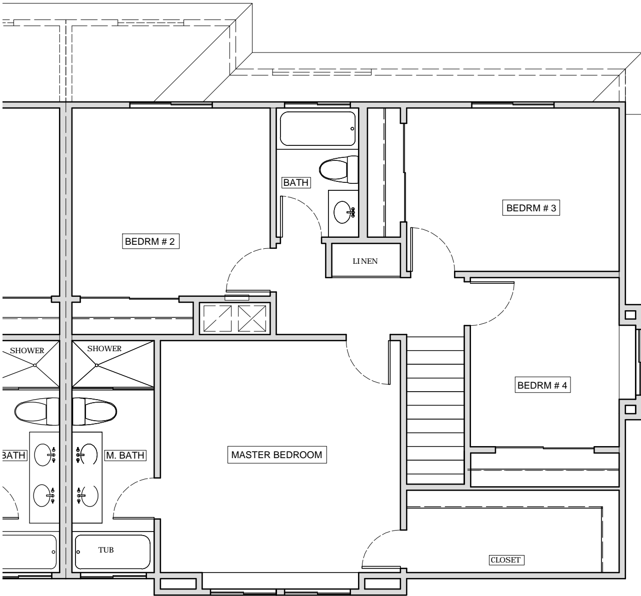
2nd. LEVEL TYPICAL END UNIT
